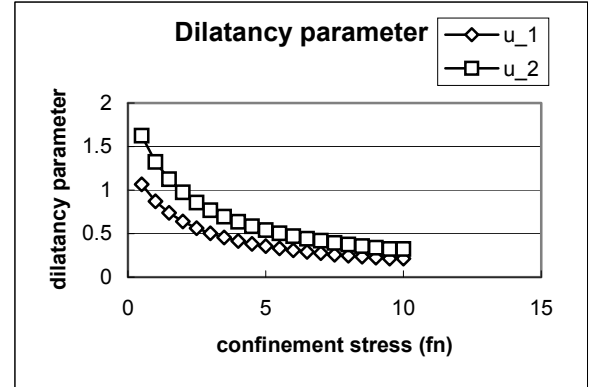
Fig. 12. Dilatancy parameters obtained by fitting the Aggregate-Interlock Relation (1981). (The symbols u_1 and u_2 represents the dilatancy parameters \mu(1) and \mu(2) respectively.)
