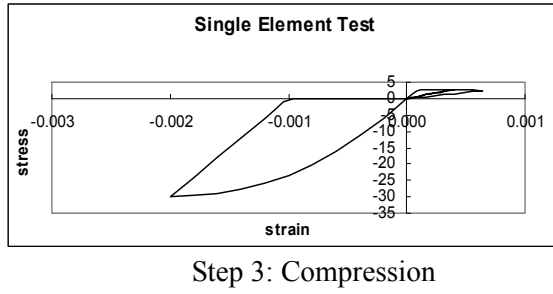
Fig. 16. Single element test (compression->tension->compression)
