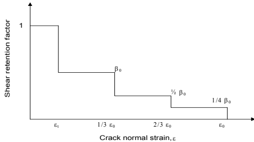
Fig. 2. shear retention factor
