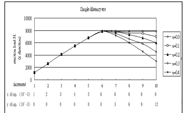
Fig. 18. Reaction load - load increment curve of simple dilatancy ( \frac{\Delta \gamma_{xy}}{\Delta \varepsilon_x} = 2.0 ) (The symbol “u” represents dilatancy parameter ( \mu_1 ))
