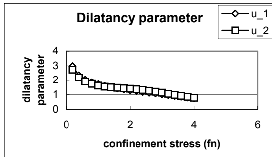
Fig. 14. Dilatancy parameter obtained by fitting the Rough Crack Model (1983) (The symbols u_1 and u_2 represent the dilatancy parameter \mu(1) and \mu(2) respectively.)
