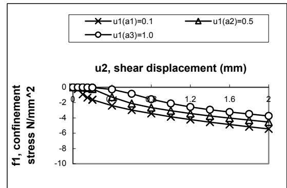
Fig. 11. Response diagram of Rough Crack Model (Gambarova and Karakoc 1983)
