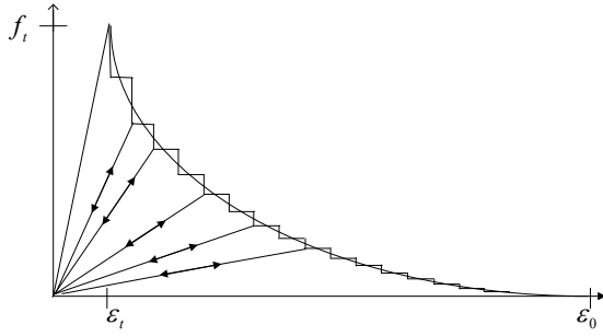
Fig. 1. Flat stepped softening curve for tension
