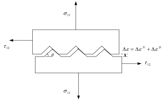
Fig. 5. A specimen subject to tensile and shear forces simultaneously Case I: Free expansion
