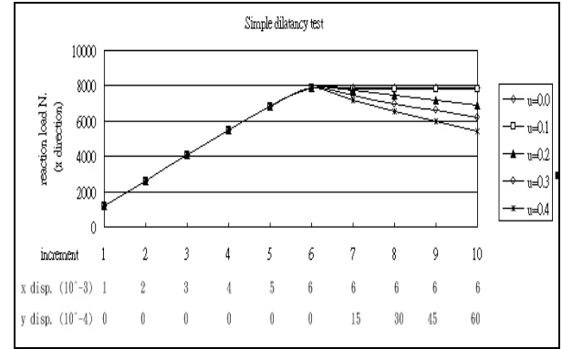
Fig. 17. Reaction load - load increment curve of simple dilatancy ( \frac{\Delta \gamma_{xy}}{\Delta \varepsilon_x} = 1.0 ) (The symbol “u” represents dilatancy parameter ( \mu_1 ))
