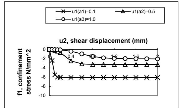
Fig. 10. Response diagram of Rough Crack Model (Bazant and Gambarova 1980)
