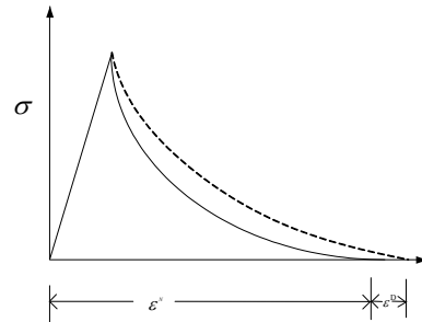
Fig. 8. Assumed strain softening curve.
