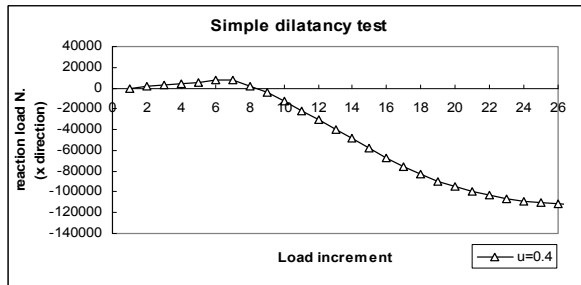
Fig. 19. Stress-strain relationship of simple dilatancy test
