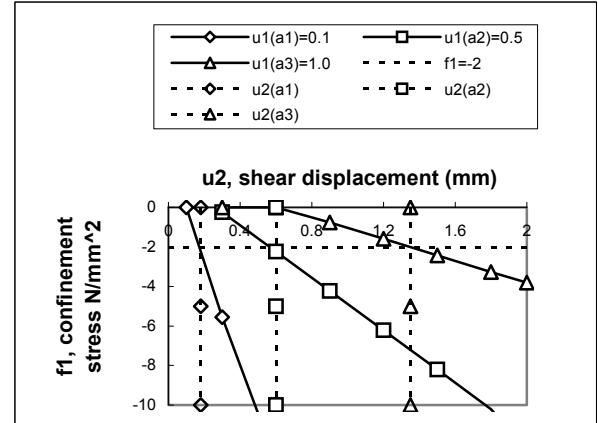
Fig. 9. Response diagram of Aggregate-Interlock Relation (Walraven and Reinhardt 1981)
