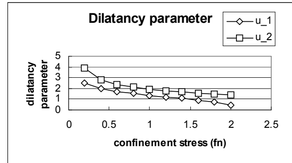
Fig. 13. Dilatancy parameter obtained by fitting the Rough Crack Model (1980) (The symbols u_1 and u_2 represents the dilatancy parameters \mu(1) and \mu(2) respectively.)
