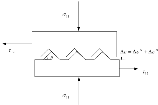
Fig. 6. A specimen subject to compressive and shear forces simultaneously Case II: Confined by boundary restraint
