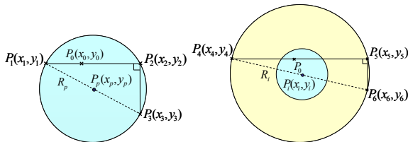
Fig. 3. Thales' theorem is applied to find (a) the inner and (b) the outer boundary of iris.
