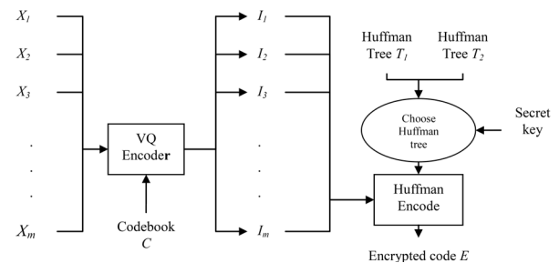
Figure 1. Batch image encryption.
