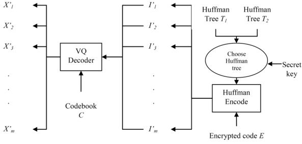
Figure 2. Batch image decryption.
