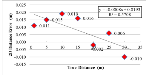
Fig. 2 Handheld laser rangefinder calibration error
